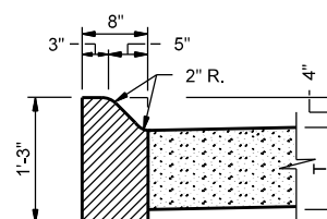
ASPHALT CURB (SLOPING)
