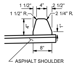
ASPHALT CURB (SLOPING)
