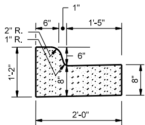
MODIFIED COMBINED CONCRETE CURB AND GUTTER (VERTICAL)
