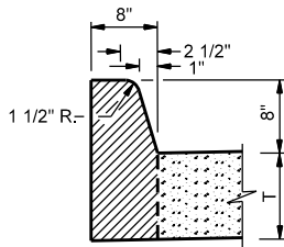
INTEGRAL CONCRETE CURB TYPE C (VERTICAL)
