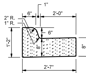
COMBINED CONCRETE CURB AND GUTTER (VERTICAL)
