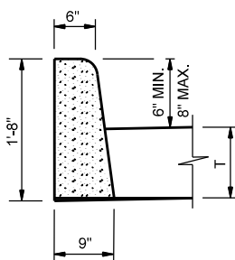
CONCRETE CURB (VERTICAL)
