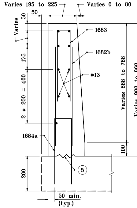
SECTION C-C
