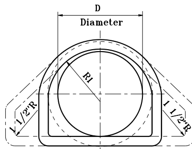
SECTION Y-Y
