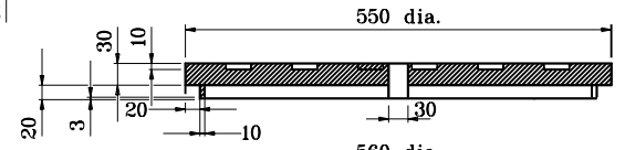
TYPE 3 RING & COVER
