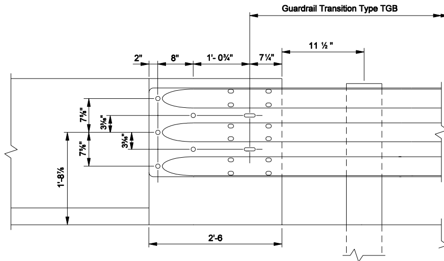
PART ELEVATION
