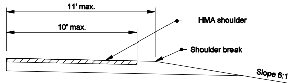
SECTION F-F
