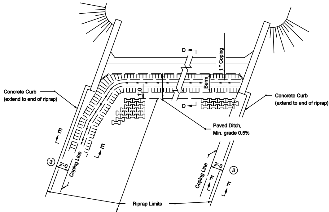
STRAIGHT WINGS
