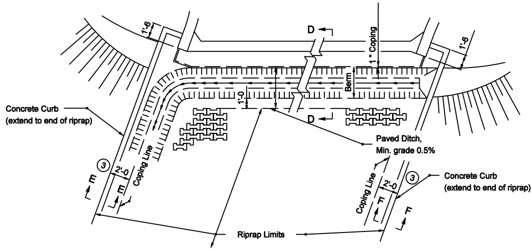
FLARED WINGS
