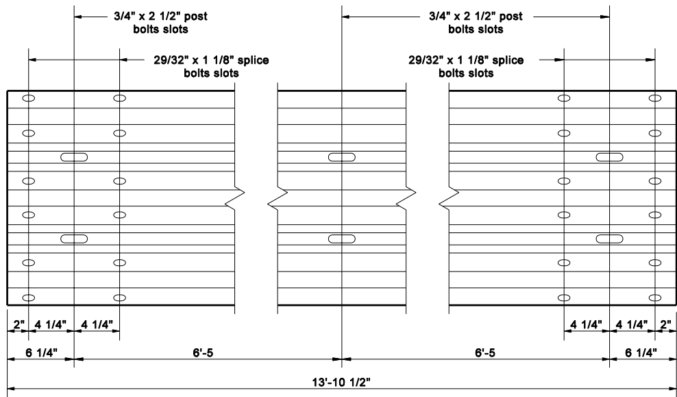
THRIE BEAM ELEVATION
