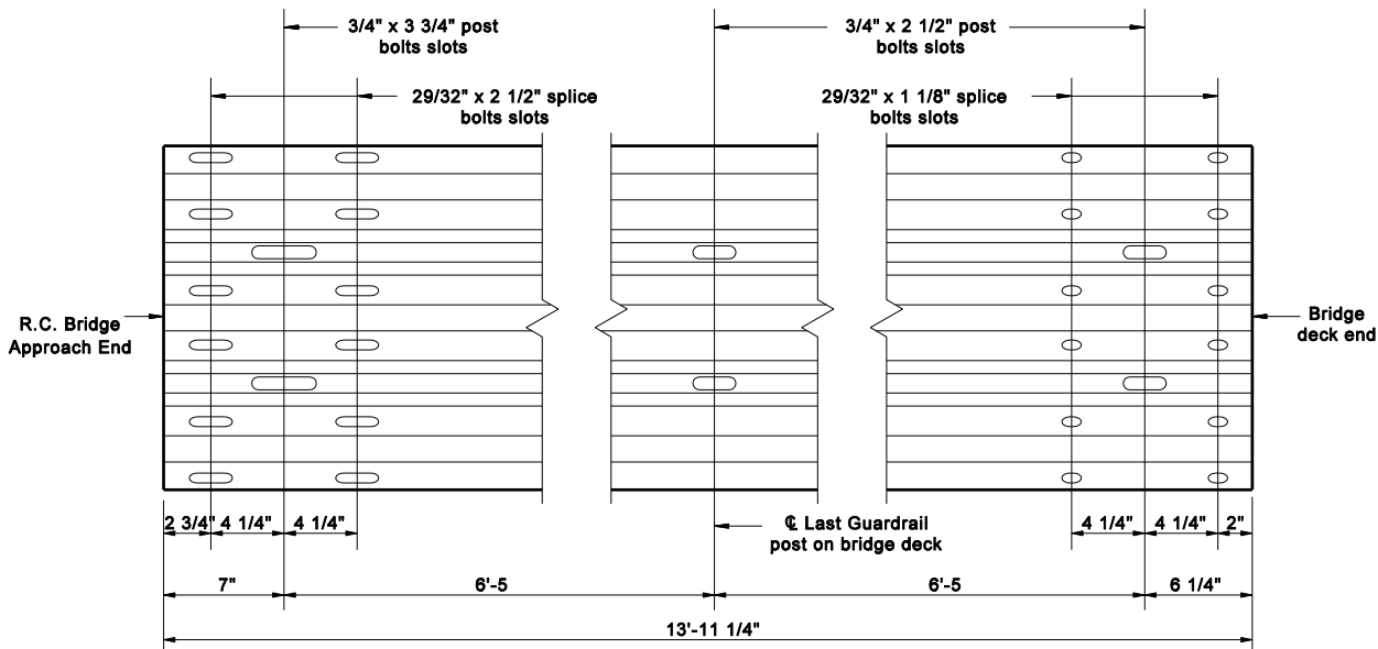
THRIE BEAM EXPANSION ELEMENT ELEVATION
