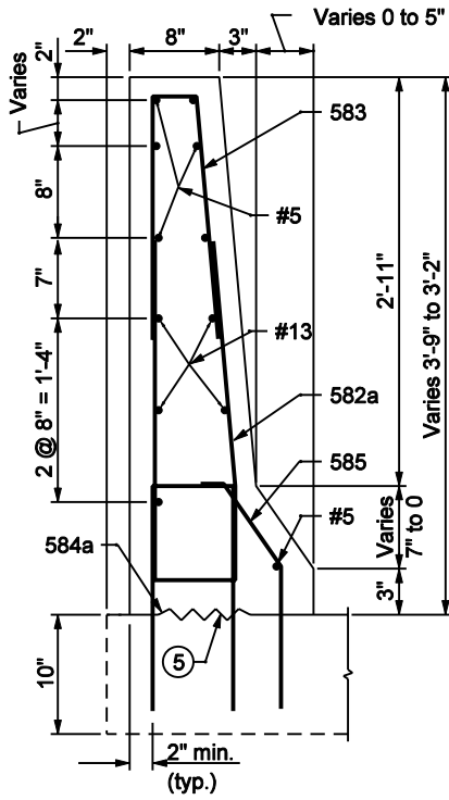
SECTION B-B
