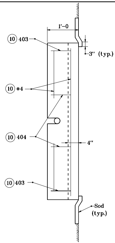
SECTION C-C
