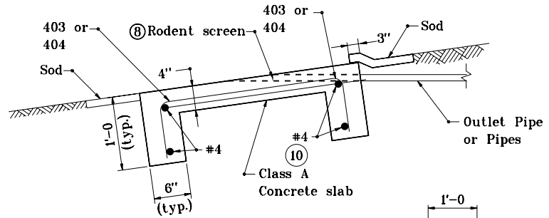
TYPICAL SECTION
