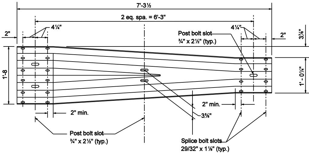
W-THRIE BEAM TRANSITION SECTION
