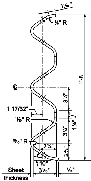
THRIE BEAM RAIL SECTION
