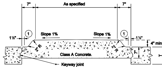
SECTION C-C
