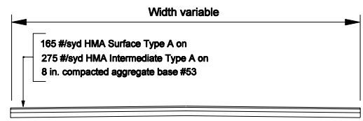
TYPICAL SECTION
