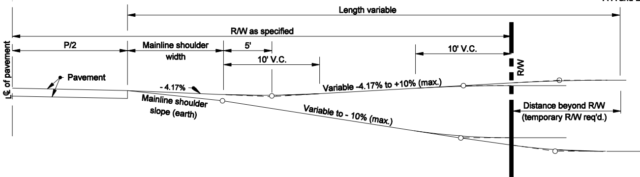
APPROACH GRADE FOR CUT OR FILL TO BE USED WITH EARTH SHOULDERS
