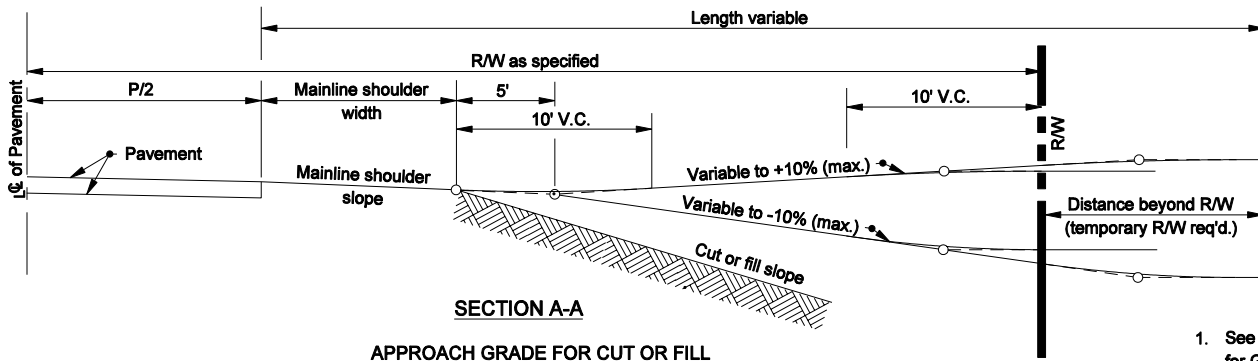
APPROACH GRADE FOR CUT OR FILL TO BE USED WITH PAVED OR COMPACTED AGGREGATE SHOULDERS
