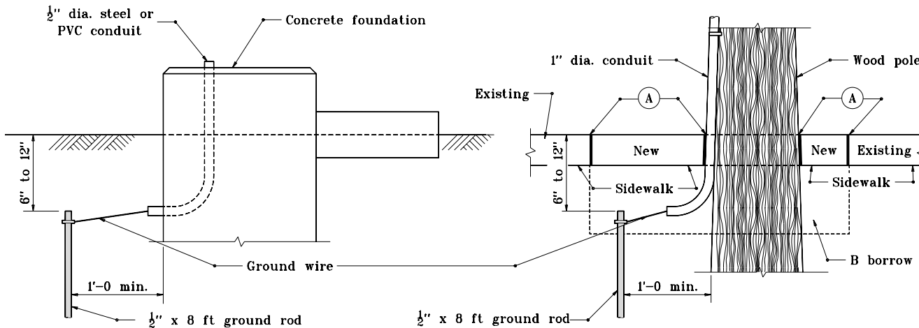
TYPICAL DETAIL GROUND ROD IN EARTH
