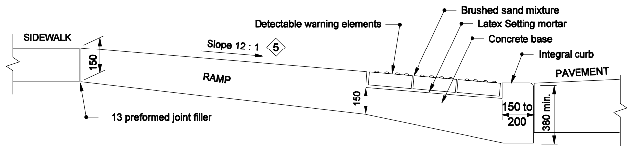
RAMP AND BRICK SURFACE CONSTRUCTION DETAIL
