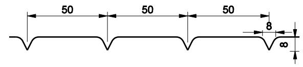
DETAIL OF RAMP GROOVES
