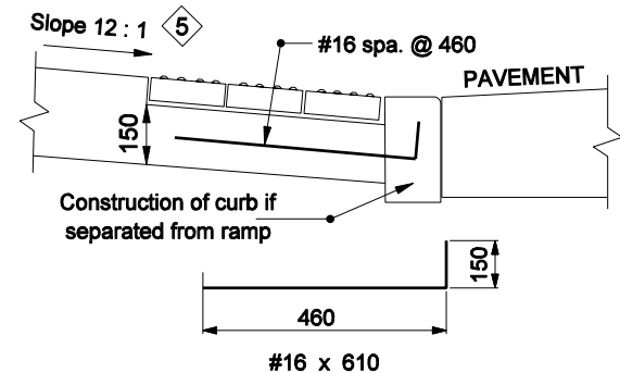
ALTERNATE CURB CONSTRUCTION
