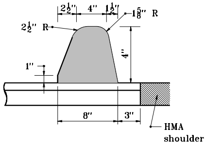
ASPHALT CURB (MOUNTABLE)
