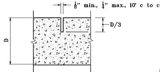
SECTION X-X
