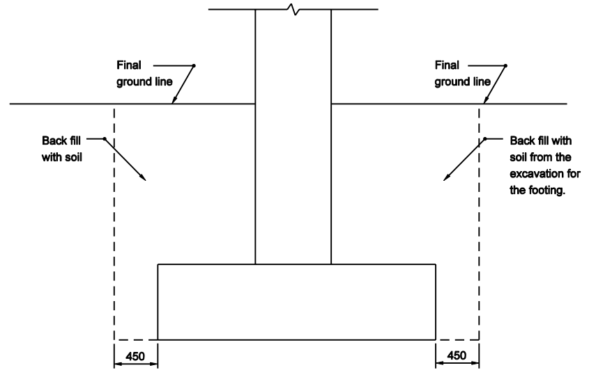
SECTION - INTERIOR BENT OR PIER For Bridge over Waterway
