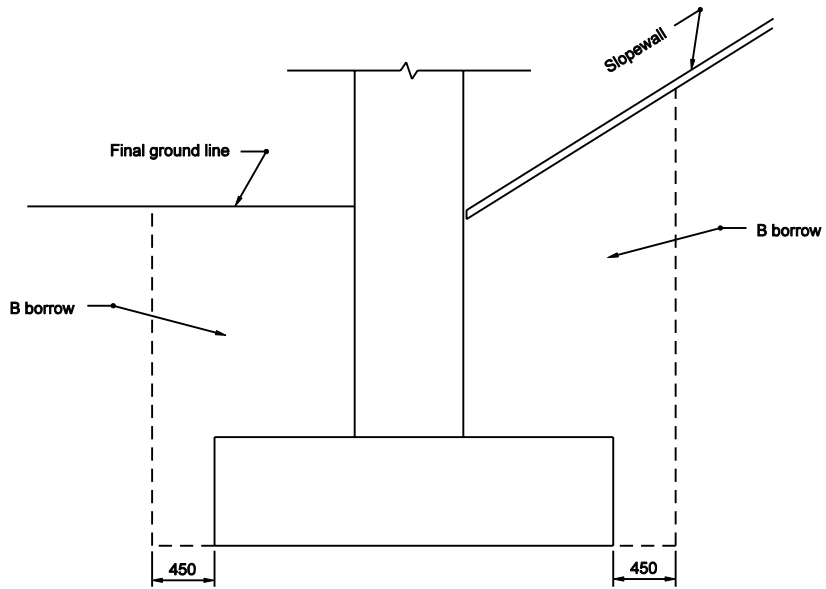
SECTION - INTERIOR BENT OR PIER Adjacent to Railroad or Highway
