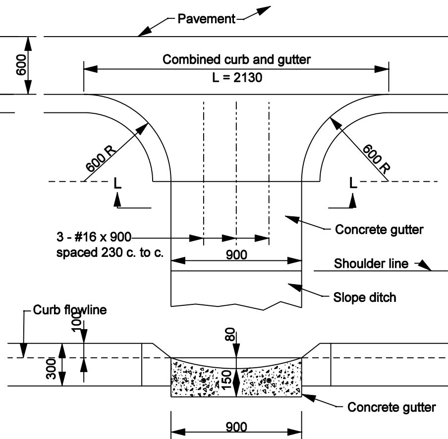
SECTION L-L
