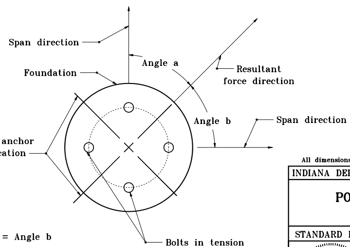
STEEL STRAIN POLE ANCHOR BOLT ORIENTATION
