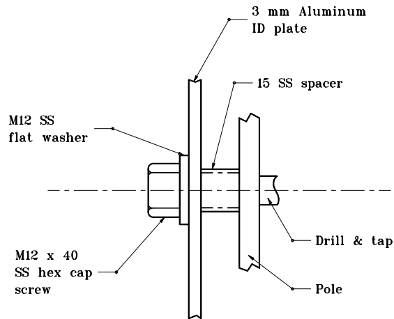
MOUNTING DETAIL
