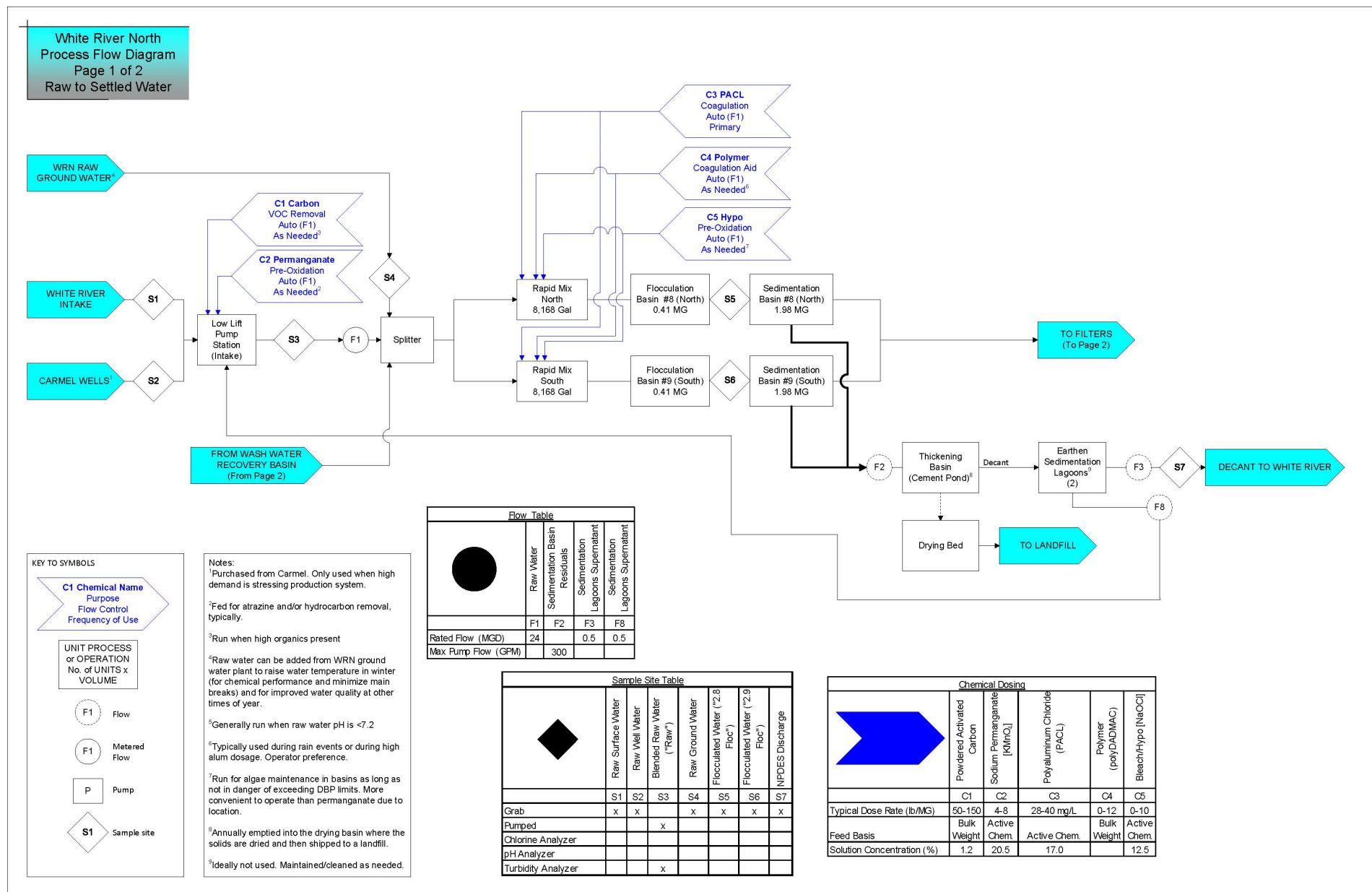
Figure 2 – Drinking Water Treatment System Flow Diagram
