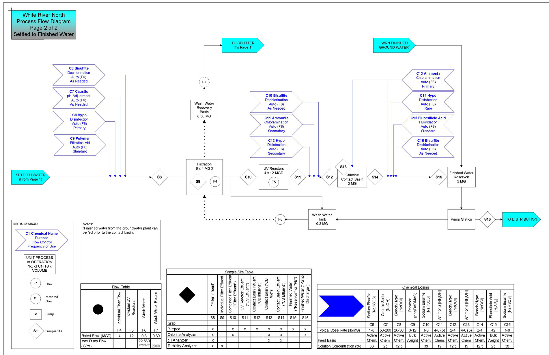
Figure 3 – Drinking Water Treatment System Flow Diagram Continue
