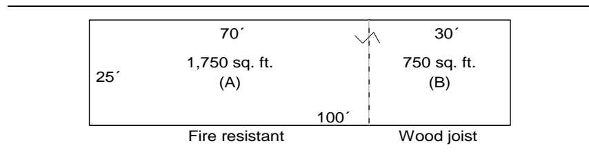
Figure 6-15. Structure with Multiple Framing Types
