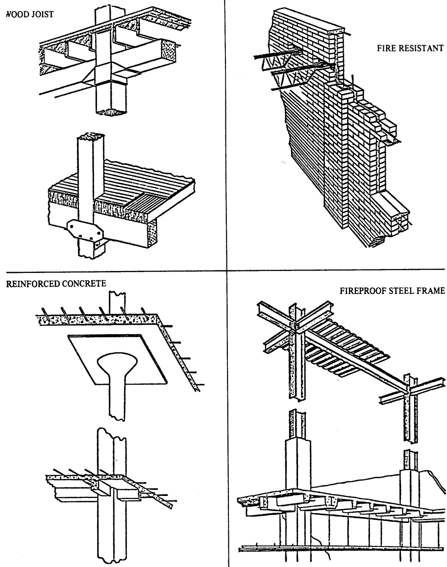
Figure 6-7. Framing Types
