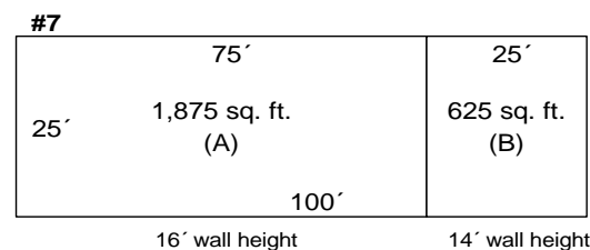
Figure 6-13. Structure with Varying Wall Heights
