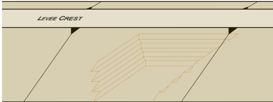
Figure 5: The excavation is backfilled and trimmed to allow topsoil placement to the design slope.
