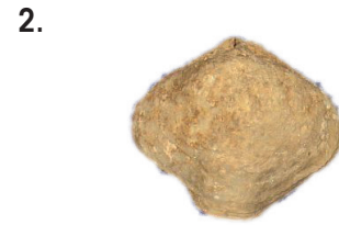
Brachiopod
