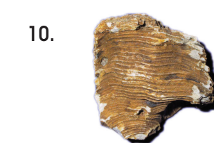
Stromatopore
