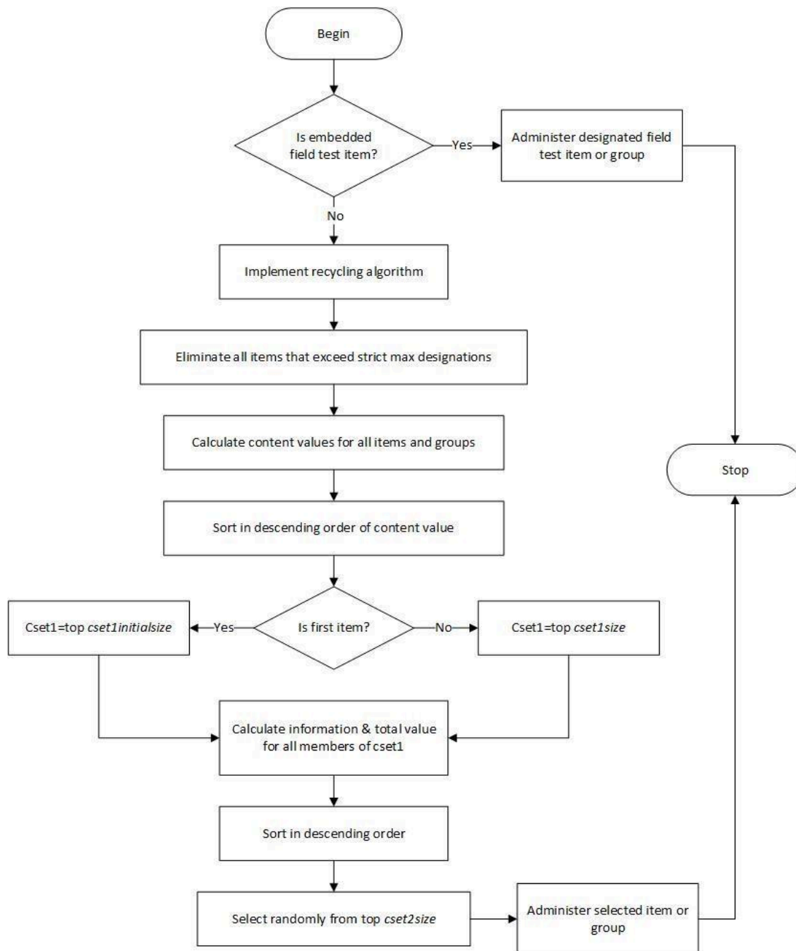
Figure 7: Summary of Item Selection Process
