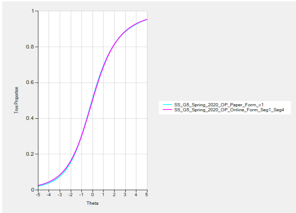
Figure 8: TCC Comparisons of Grade 5 Social Studies Online and Paper Forms
