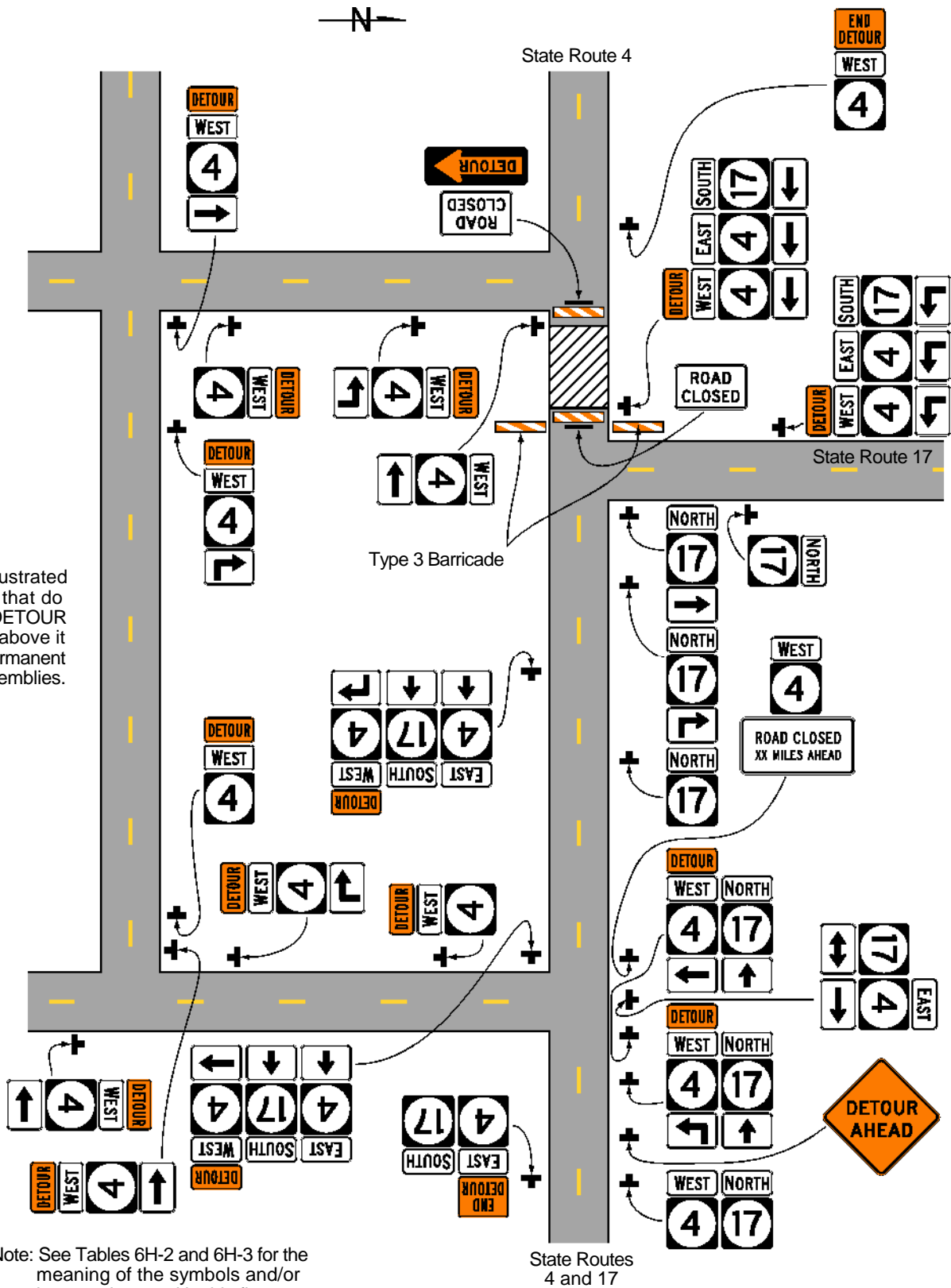
Figure 6H-9. Overlapping Routes with a Detour (TA-9)
