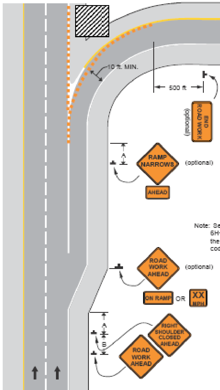
Figure 6H-43AY. Partial Exit Ramp Closure with Work in Gore Area (TA-43AY)
