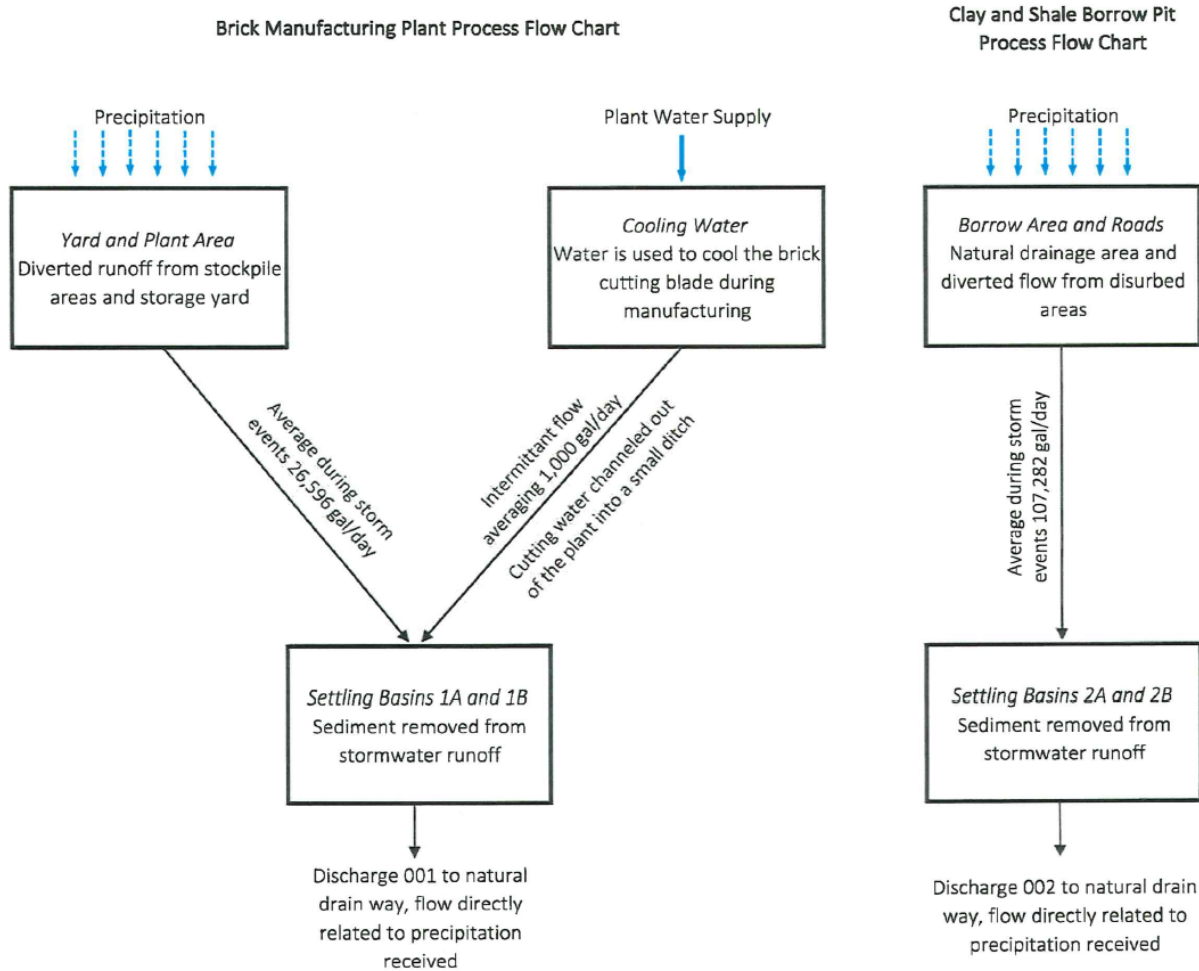
Figure 2: Water Balance Diagram
