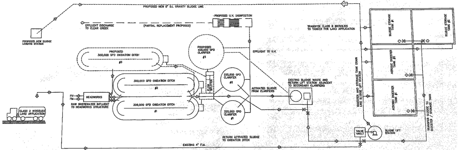
1 WWTP HYDRAULIC SCHEMATIC 2 NO SCALE
