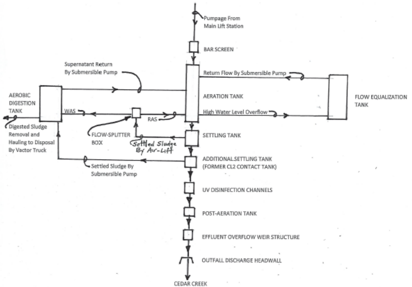
SCHEMATIC FLOW DIAGRAM WASTEWATER TREATMENT PLANT LAKE DALECARLIA REGIONAL WASTE DISTRICT Prepared By: Haas & Associates, LLC Date: January 2, 2020
